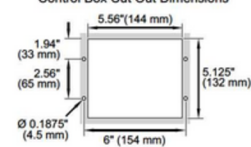
Control Box Cut Out Dimensions
